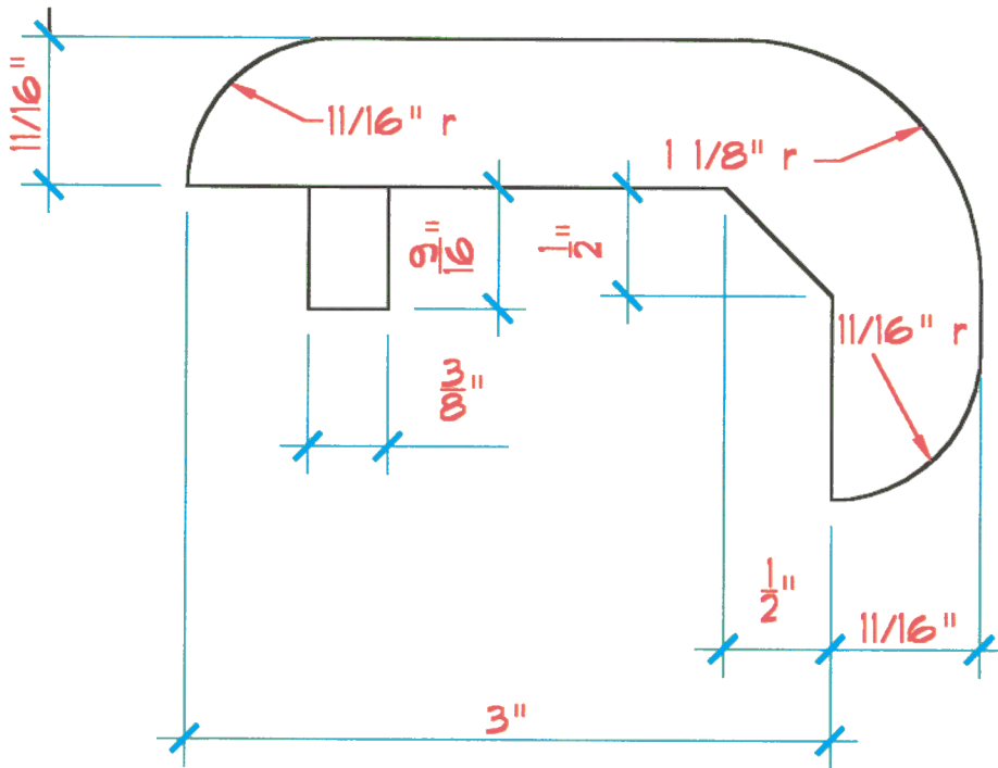
Flat Bar - .5" Bevel Corner "FB.5B"
