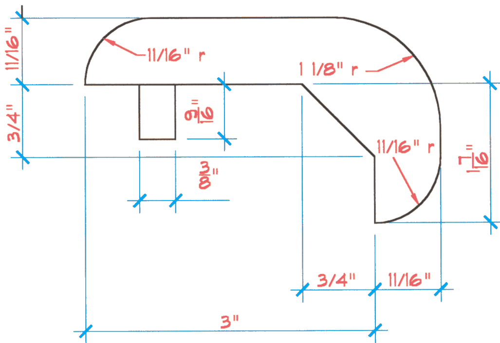
Flat Bar - 0.75" Bevel Corner "FB.75B"
